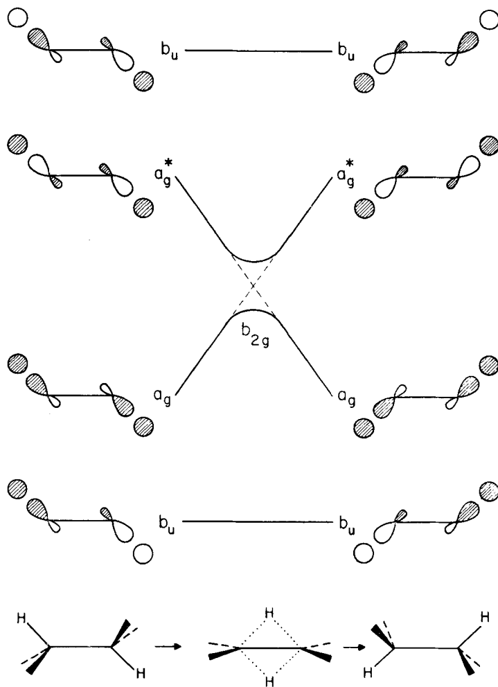
Fig. 3. Level correlation diagram for the rearrangement 1 \rightarrow 1'
