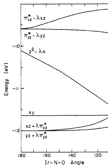
Figure 3. Calculated energy levels of \text{IrCl}_4\text{NO}^{2-} as a function of the Ir-N-O angle. The labels identify the primary character of the MO, even though these orbitals are to various degrees delocalized.
