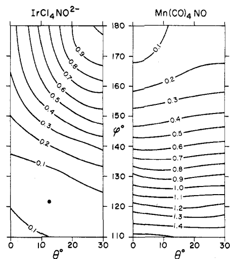
Figure 7. Calculated potential energy surfaces for Berry pseudorotation and bending in IrCl_4NO^{2-} and Mn(CO)_4NO . The angles \theta and \phi are described in the text and structure 24. The energy contours are in electron volts relative to the minimum energy points of the graph: \phi = 180^\circ, \theta = 0^\circ for Mn(CO)_4NO , the dark dot for IrCl_4NO^{2-} .
